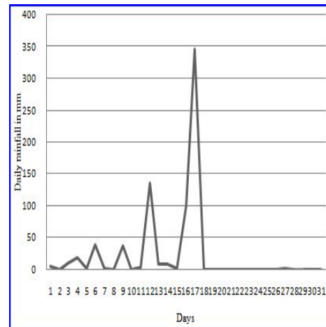
Figure 8: Ratnapura district daily rainfall variation in May 2003
