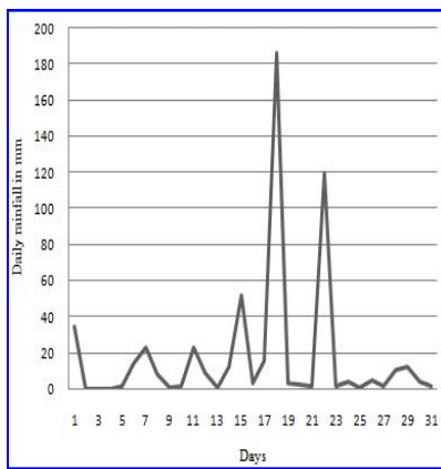
Figure 41: Daily rainfall variation in July 2008 in Ratnapura district.
