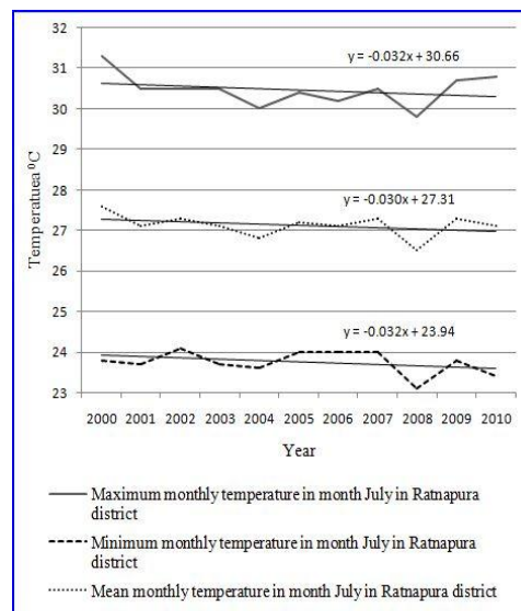
Figure 4: Maximum, Minimum and Mean monthly temperature variation in month July during last decade in Ratnapura district
