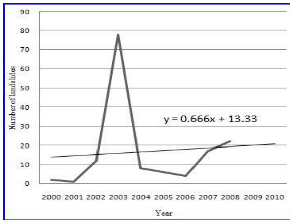
Figure 5: Landslide frequency in Ratnapura district during the last decade.
