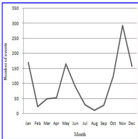
Figure 6: Seasonal Distributions of Landslides in Sri Lanka: 1974 - 2008(Sri Lanka National Report on Disaster Risk, Poverty and Human Development Relationship, 2009).
