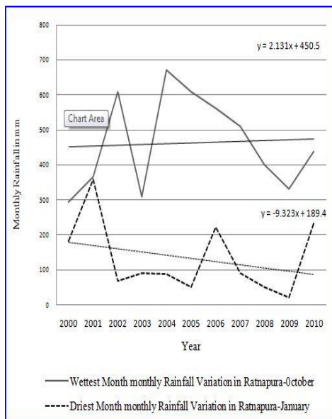
Figure 2: Wettest month and driest month monthly rainfall variation in Ratnapura district during last decade
