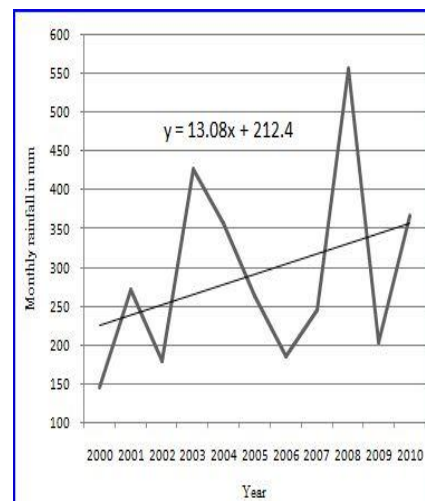
Figure 10: Monthly rainfall variation in month July during last decade in Ratnapura district.
