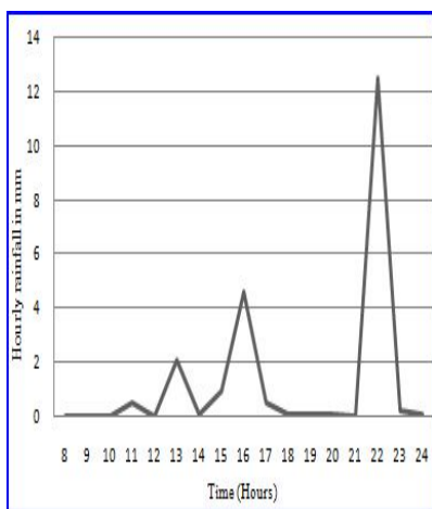
Figure 12: Hourly rainfall variation in 21st of July 2008 in Ratnapura district.
