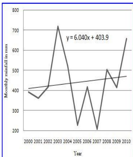
Figure 7: Monthly rainfall variation in month May during last decade in Ratnapura district
