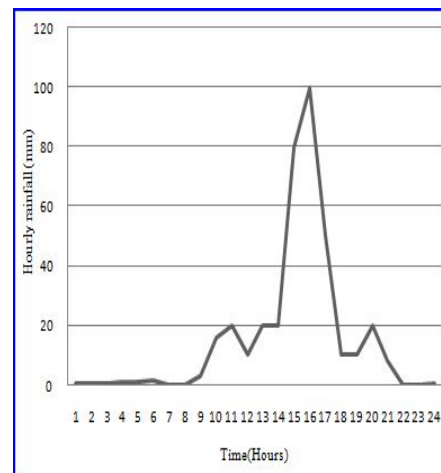
Figure 9: Hourly rainfall variation on 17th May 2003 in Ratnapura district
