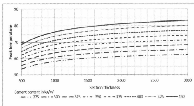
Figure 12: Peak temperature variation of various concrete mixes with a placing temperature of 32°C and 25% fly-ash
