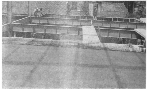
Figure 7: Pre-cast Pre-tensioned slabs spanning on steel beams with a reinforced in-situ topping on top
