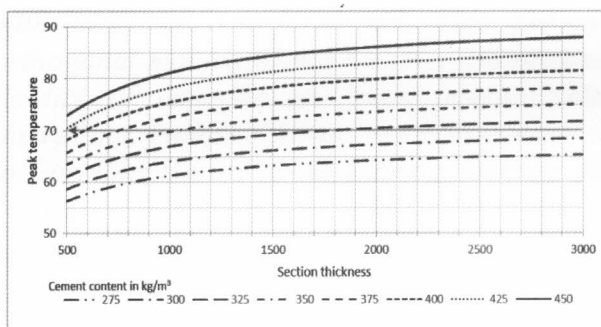
Figure 11: Peak temperature variation of various concrete mixes with a placing temperature of 32°C and 15% fly-ash
