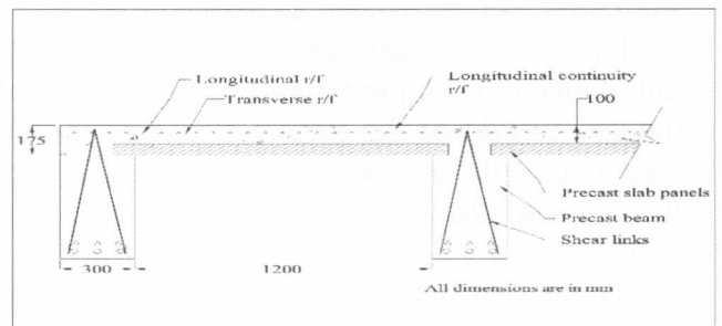
Figure 5: The cross section of the beam slab system
