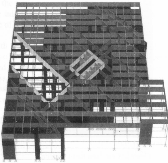
Figure 4: SAP 2000 model of the Cellular transfer plate of the Sky Garden Building
