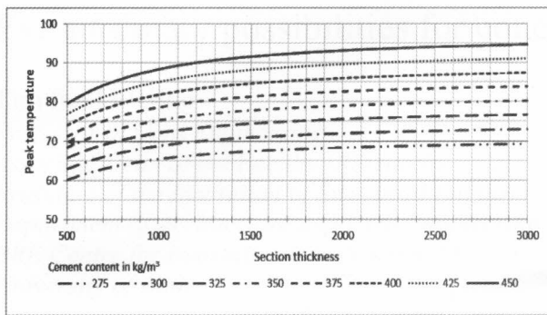
Figure 10: Peak temperature variation of various concrete mixes with a placing temperature of 32°C and 0% fly-ash
