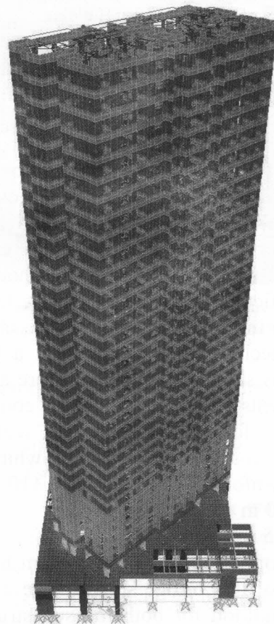
Figure 3: SAP 2000 analysis model of the Sky Garden Building
