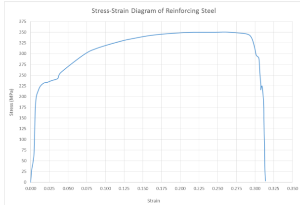
Figure 2. Stress-Strain Diagram of Reinforcing Steel
