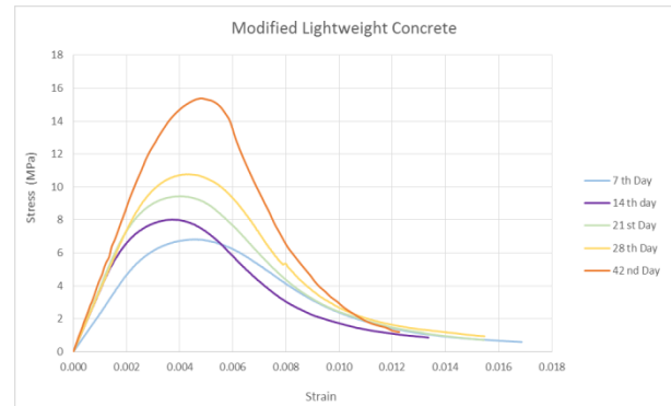
Figure 6. Stress-Strain diagram of Unconfined Modified Lightweight Concrete
