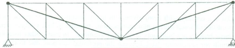
6(b). POLYGONAL TENDON
