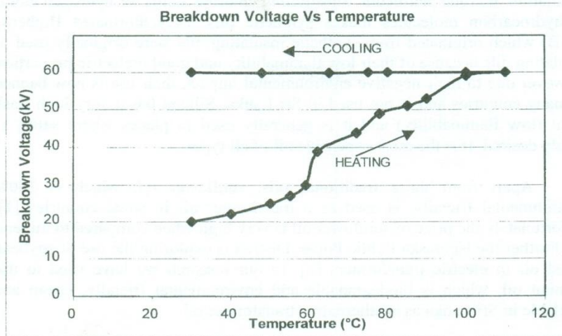
Figure 2 - Heating/Cooling Curve of Coconut Oil.
