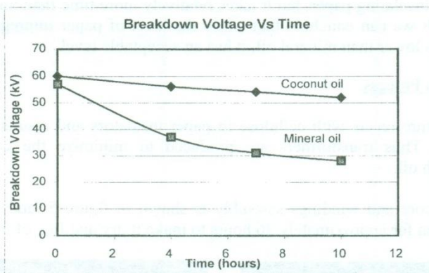
Figure 3 - Moisture Absorption of Oil
