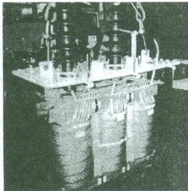
Figure 5-Core and Winding Assembly
