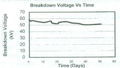
Figure 10 - Degradation of oil
