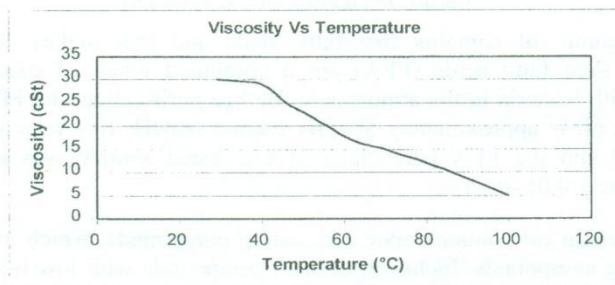
Figure 8- Variation of Viscosity of Coconut Oil.
