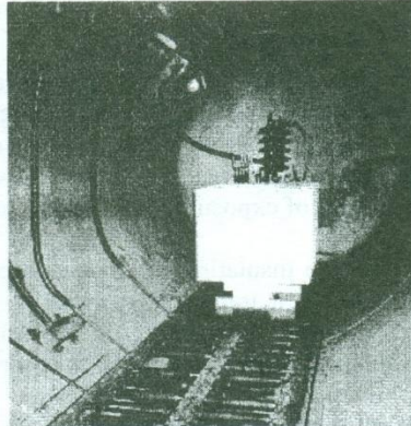
Figure 6-Vacuum Impregnation
